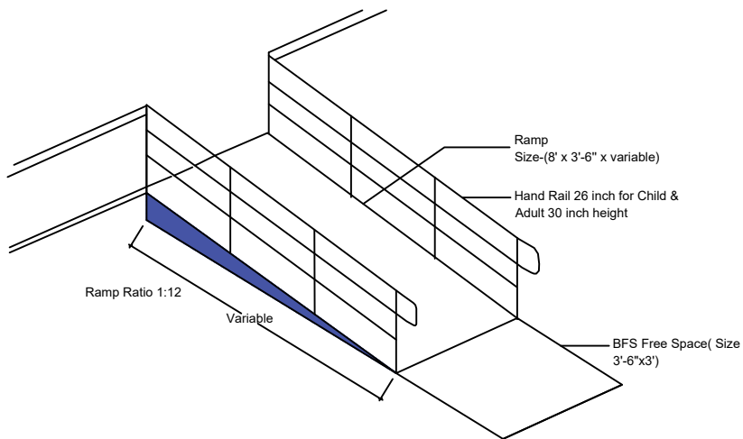
Isometric View of Ramp
