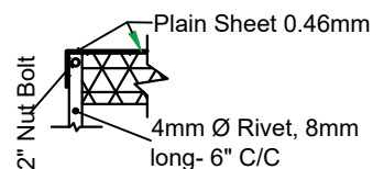
Section Z: Plain Sheet 0.46mm for roof & fixed with rivet
