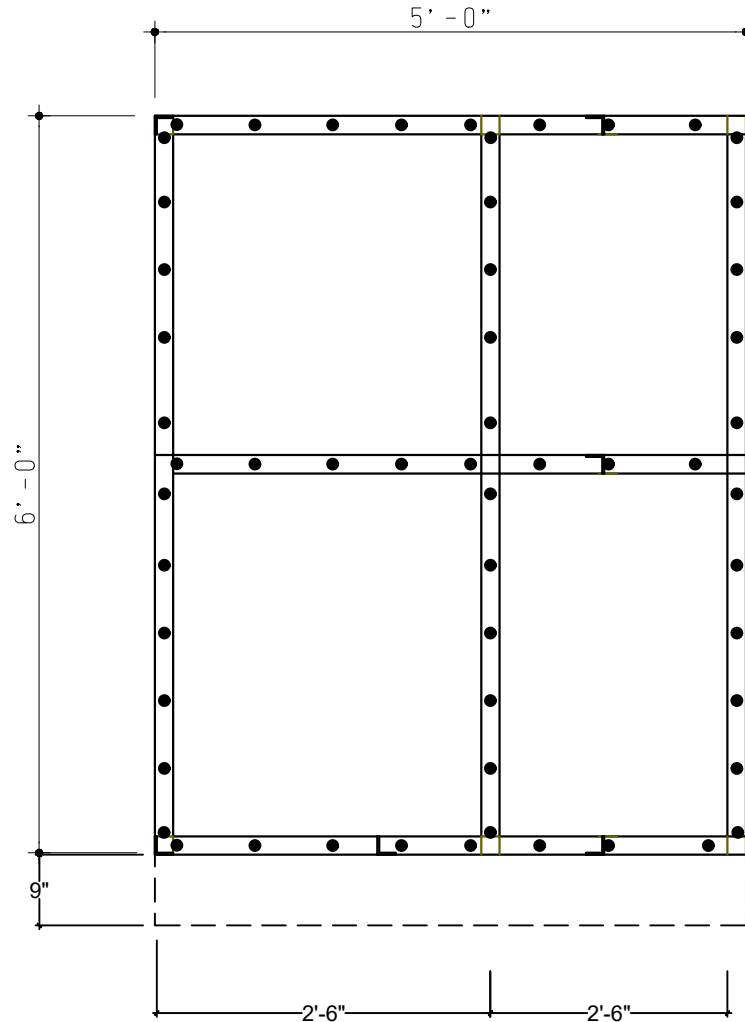
Roof View
