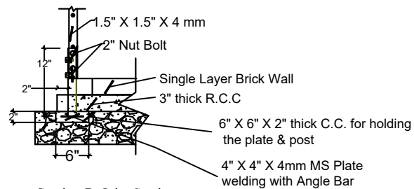
Section P: Joint Section
