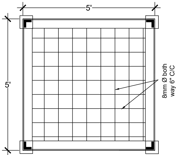
Section: Reinforcement Details of Slab
