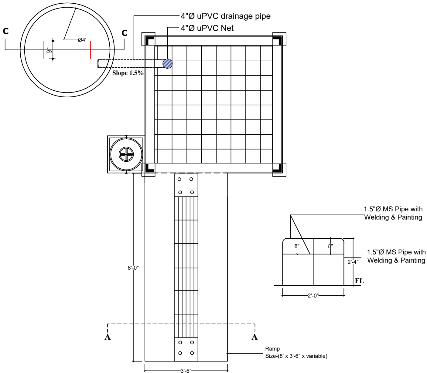
PLAN OF BATHING WITH SOAK PIT (STEEL FRAME)
